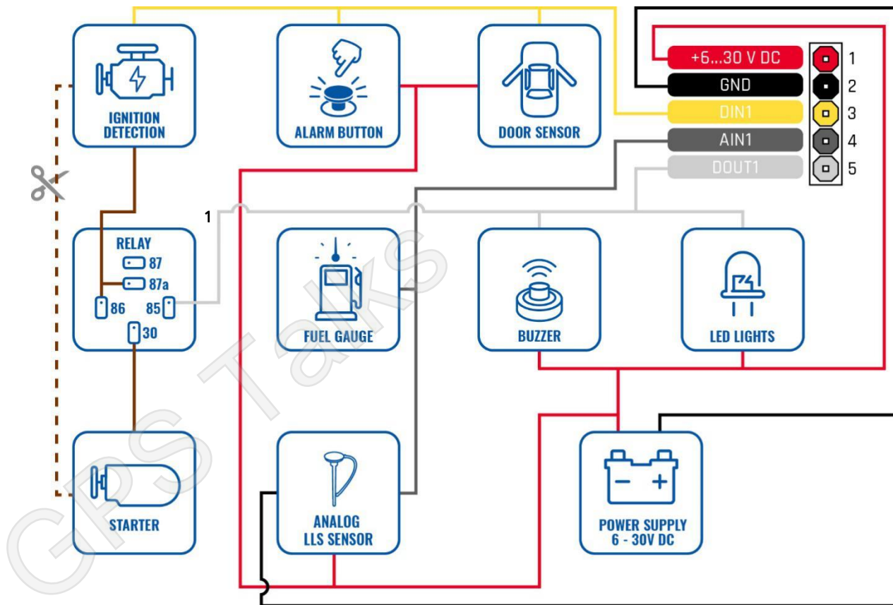
Figure 3 FMB910 Wiring scheme
