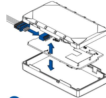
2 Figure 5 Wiring harness connection
